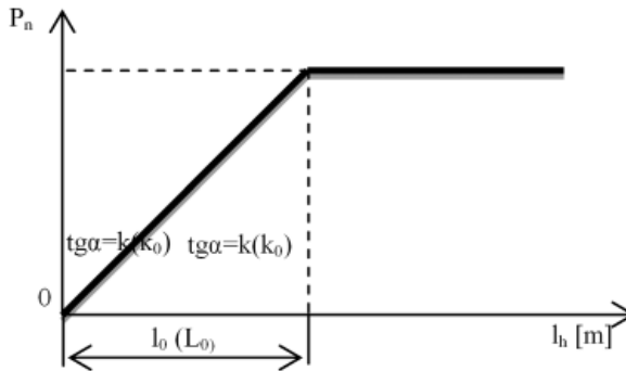
Fig. 3. Dynamic characteristic of braking systems: l_0 (L_0) – distance of braking force increase: K_{(k_0)} – coefficient expressing the braking force increase, t_0 (T_0) – time of braking force increase over the distance l_0 (L_0) , P_h – braking force, l_h – braking distance
