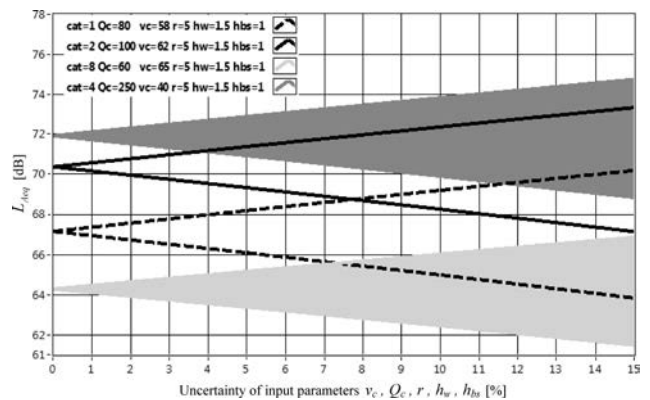
Fig. 1. Variability range of the estimated sound levels in dependence on the uncertainty of input parameters.
