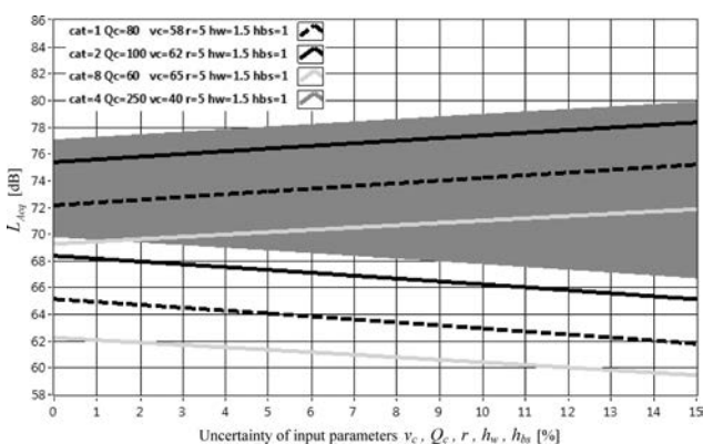
Fig. 2. Variability range of the estimated sound level in dependence on the input parameters uncertainty when taking into account the variability of the C_{b,c} parameter
