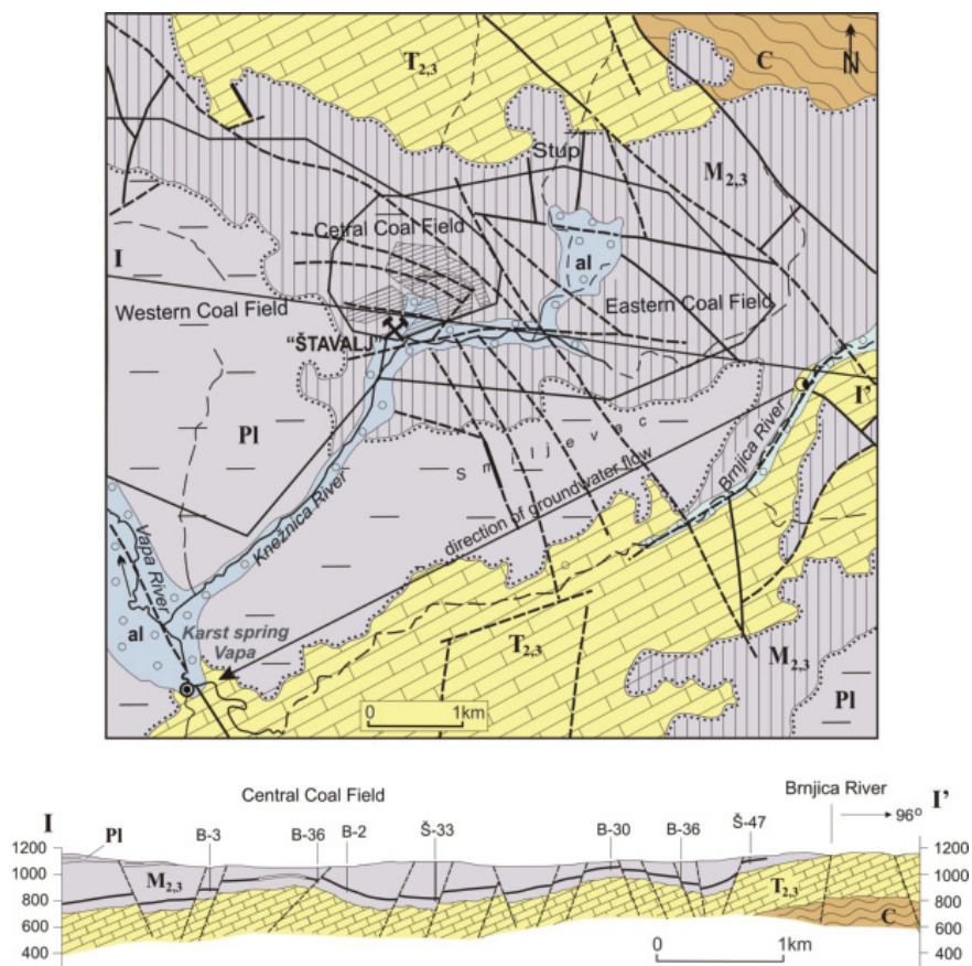
Fig. 2. Hydrogeological map of the extended area of the Štavalj Coal Mine, including characteristic section I-I' al – alluvium, intergranular aquifer; Pl – Pliocene gravel, sand and clay, hydrogeological complex; M_{2,3} – Miocene marl, marly limestone, clay and coal, hydrogeological complex; T_{2,3} – Middle and Upper Triassic limestones, karst aquifer; C – Carboniferous schists, non hydrated rocks
